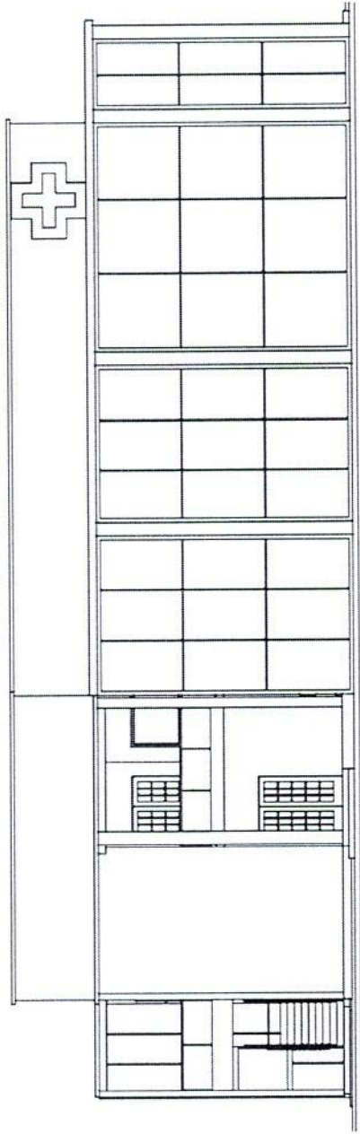
FRONT ELEVATION
